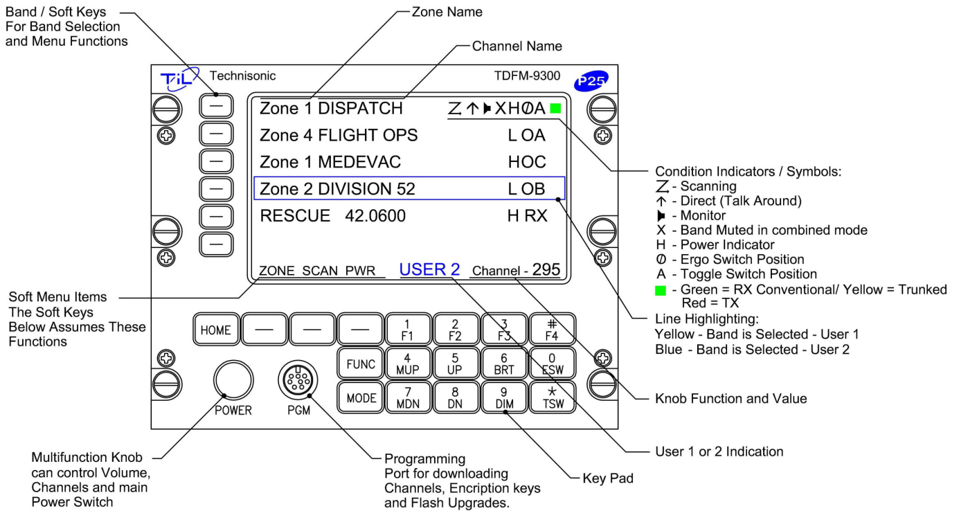
FIGURE 1: Front Panel Controls – TDFM-9300 Transceiver
